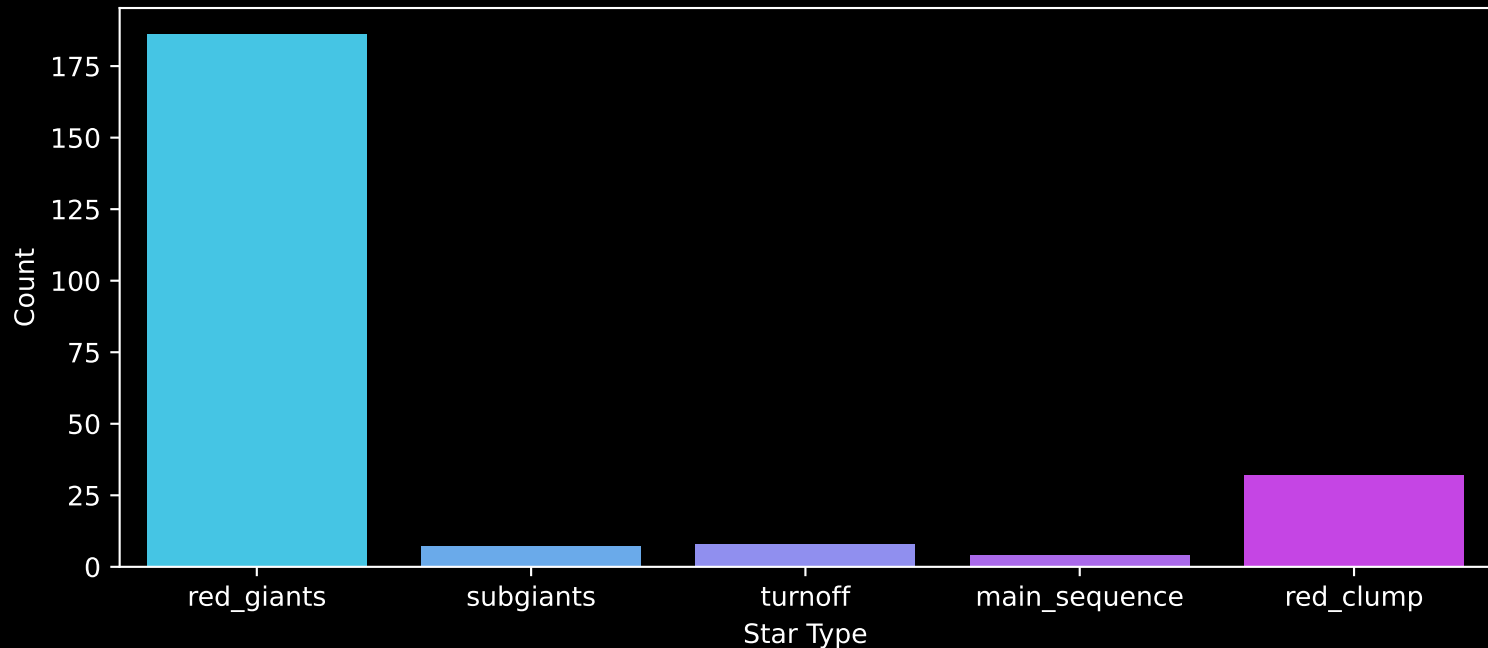
APOGEE DR17 Field: [N6388] Count plot of Star Type
