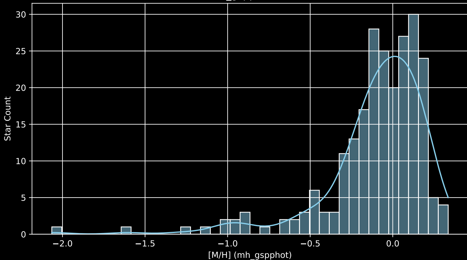
APOGEE DR17 Field: [N6388 [M/H] (mh_gspphot) (n= 235)
