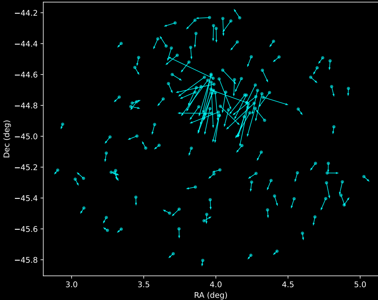
APOGEE DR17 Noise Stream Proper Motion Vectors (n=134)
