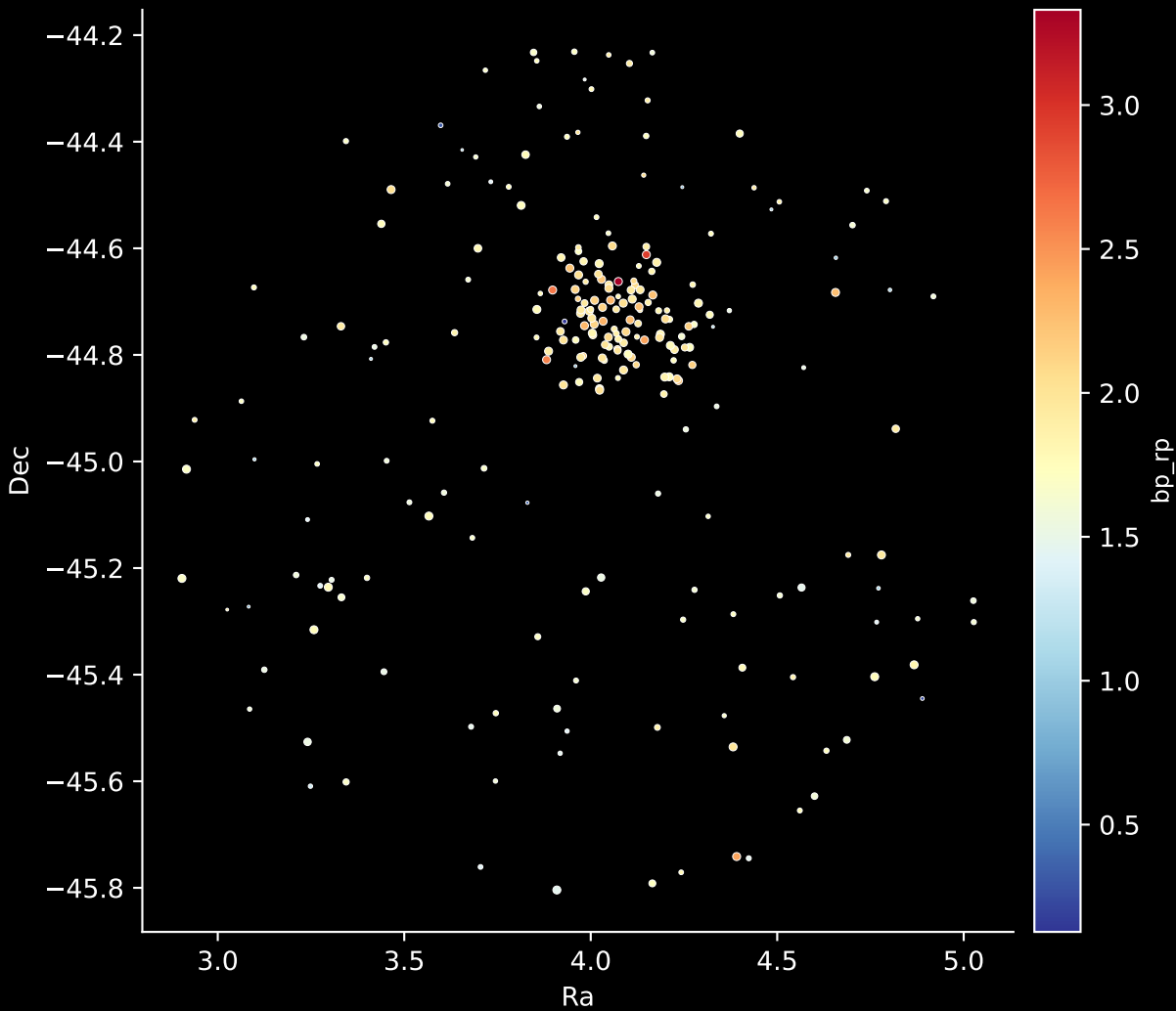
APOGEE DR17 Field: [N6388] Stars: 237
