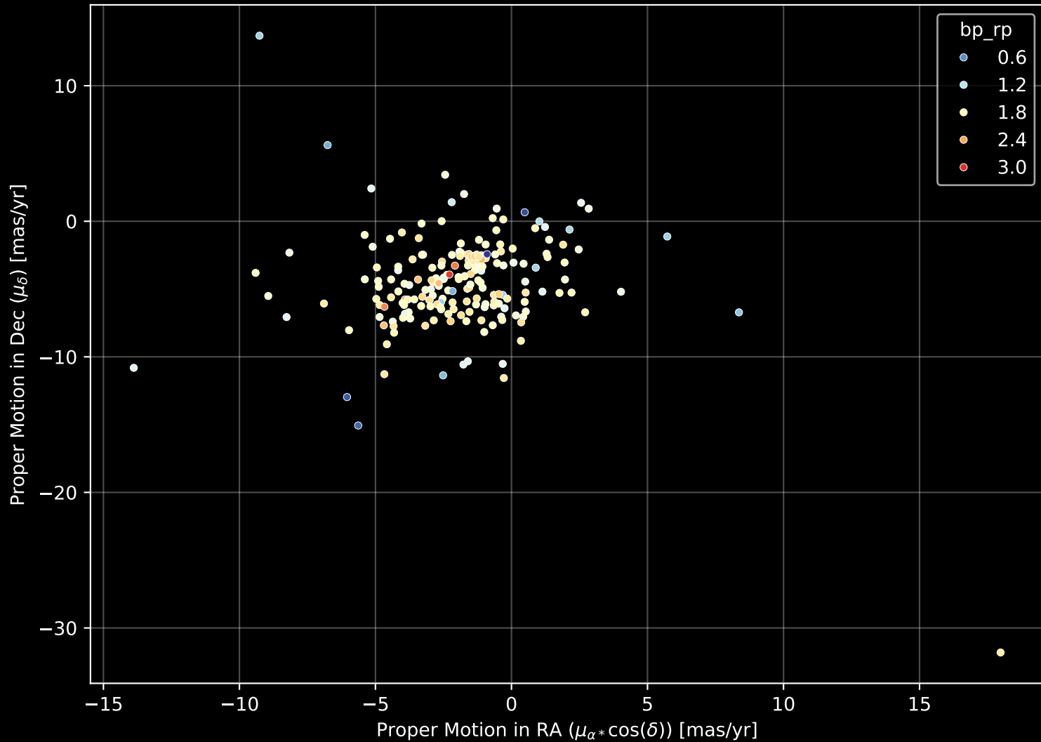
APOGEE DR17 Field: [N6388] Proper Motion Diagram (n= 237)
