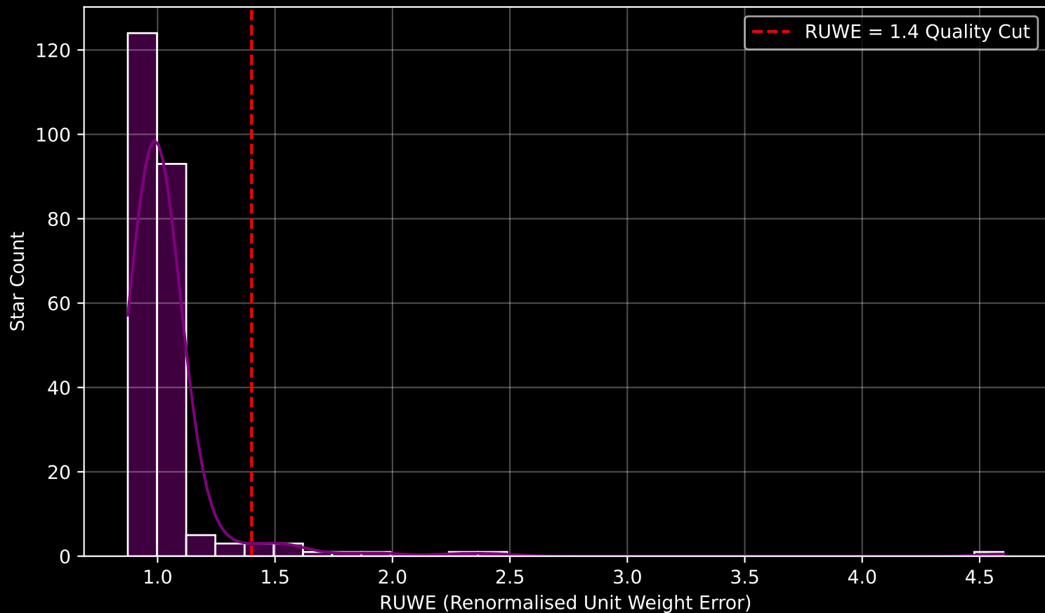
GAPOGEE DR17 Field [N6388] RUWE Distribution (n= 237)
