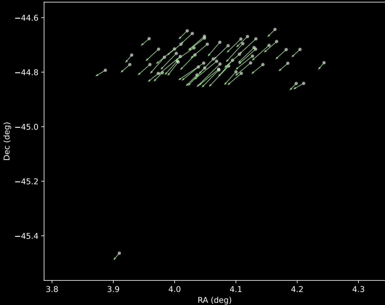
APOGEE DR17 Cluster 5 Proper Motion Vectors (n=57)
