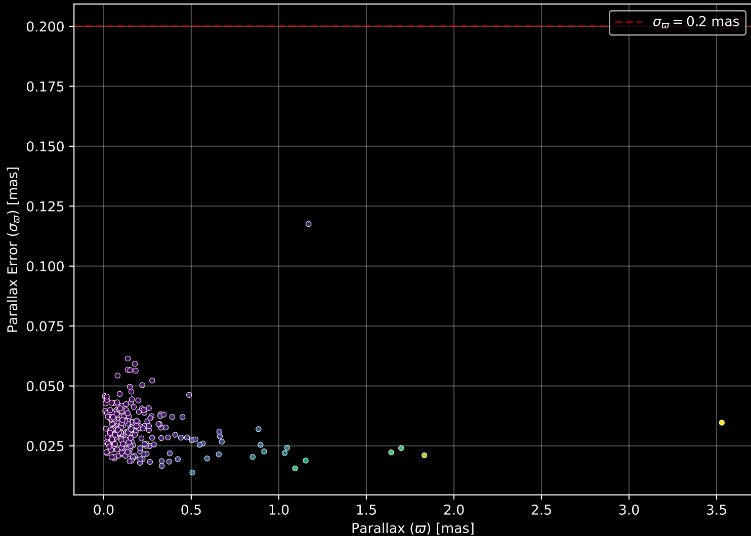
APOGEE DR17 Field: [N6388] Parallax Quality (n= 237)
